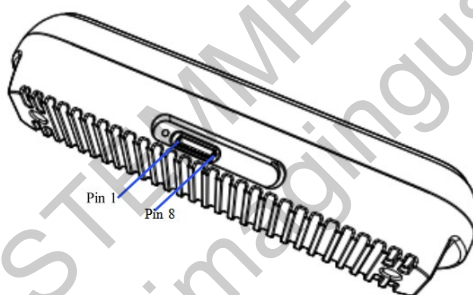
Gemini 335Lg Multi-device Synchronization Pin Placement.
